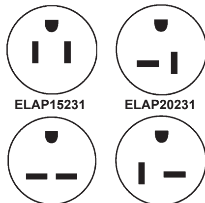
ELAP15231 ELAP20231 ELAP15232 ELAP20232 Explosion-Proof Plugs
