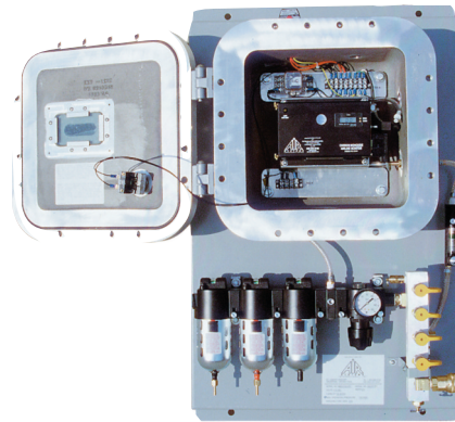
Explosion-Proof Grade-D Custom Filtration Panel B50-COPMEX
